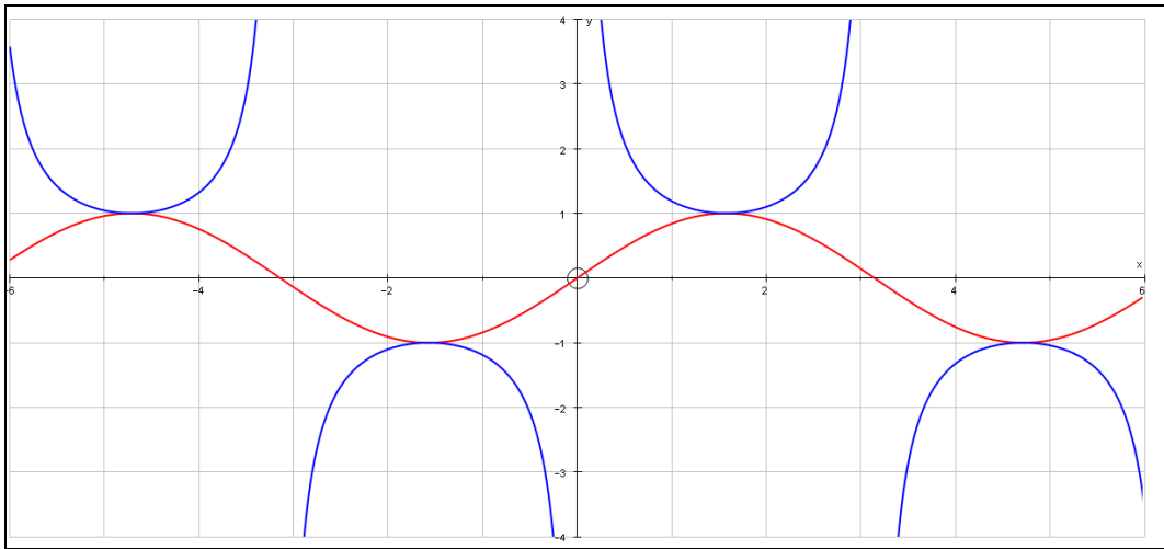
y = \sin x and y = \operatorname{cosec} x
