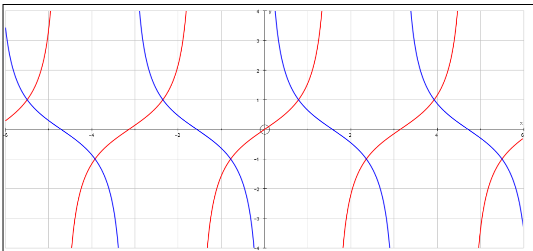
y = \tan x and y = \cot x
