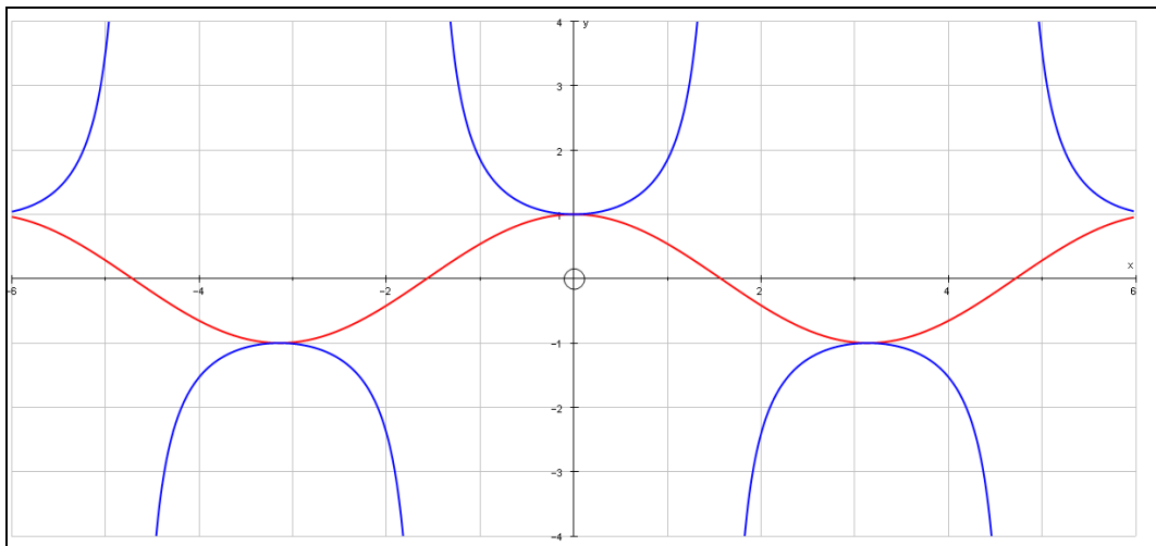
y = \cos x and y = \sec x
